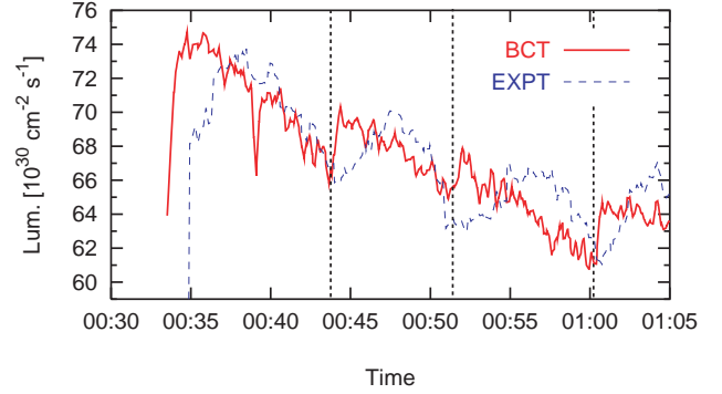
Figure 3: Comparison of the average luminosity from the experiments (EXPT) and the beam lifetime (BCT).
