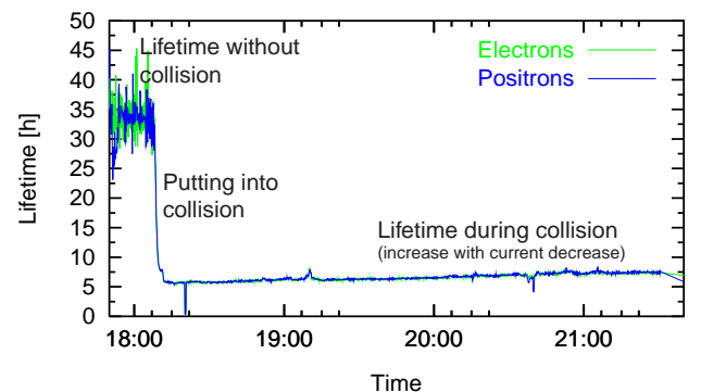
Figure 1: Evolution of beam lifetime in LEP.
