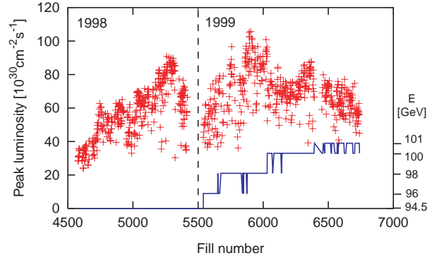
Figure 3: Peak luminosity in all physics fills in 1998 and 1999. The line indicates the beam energy.
